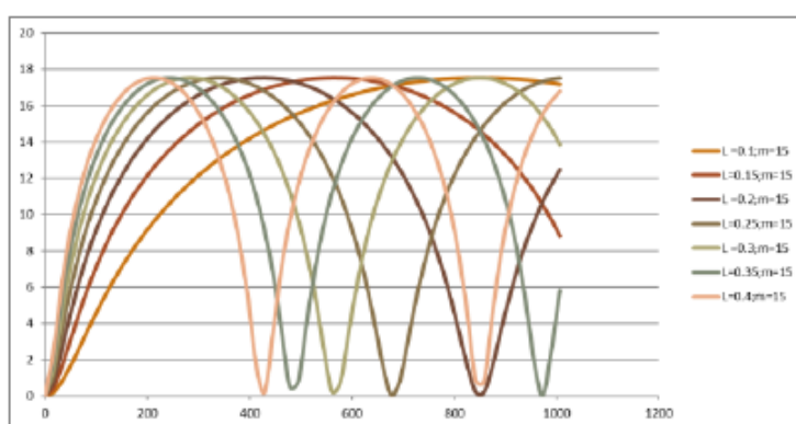
Chart 4–TLvsFrequency(m=15)
