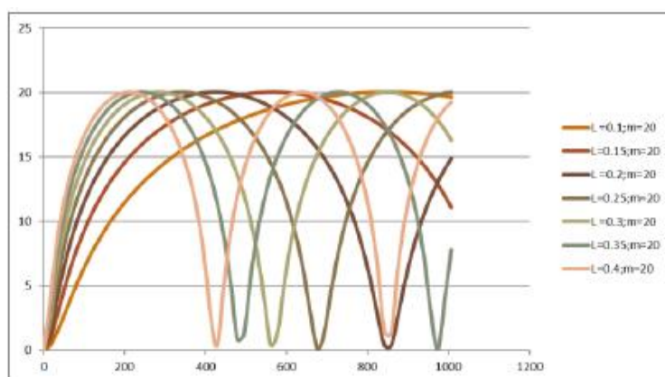
Chart 5 – TL vs Frequency (m = 20)
