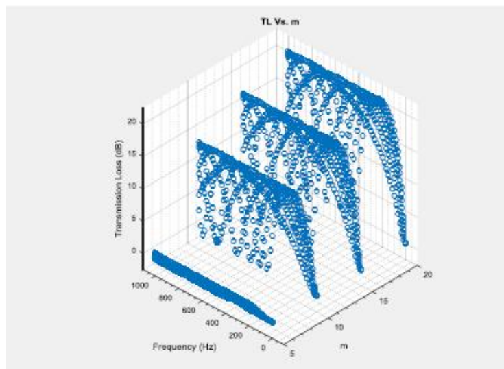
Chart 7 – TL vs Frequency vs Expansion ratio
